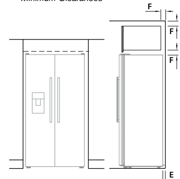
Minimum Clearances
